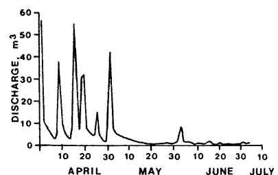
FIGURE 2. Mean daily discharge recorded at Kilometer 76.
